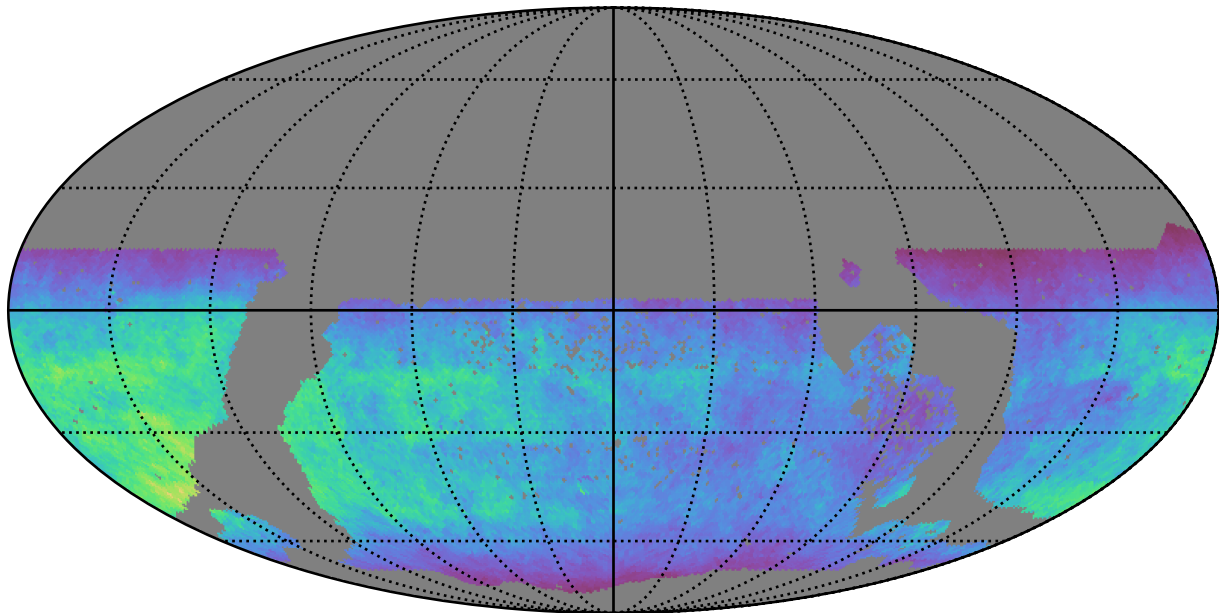
too_elab_r32_d3_ugrizy_v3.4_10yrs WFD u band: Normalized Teff
