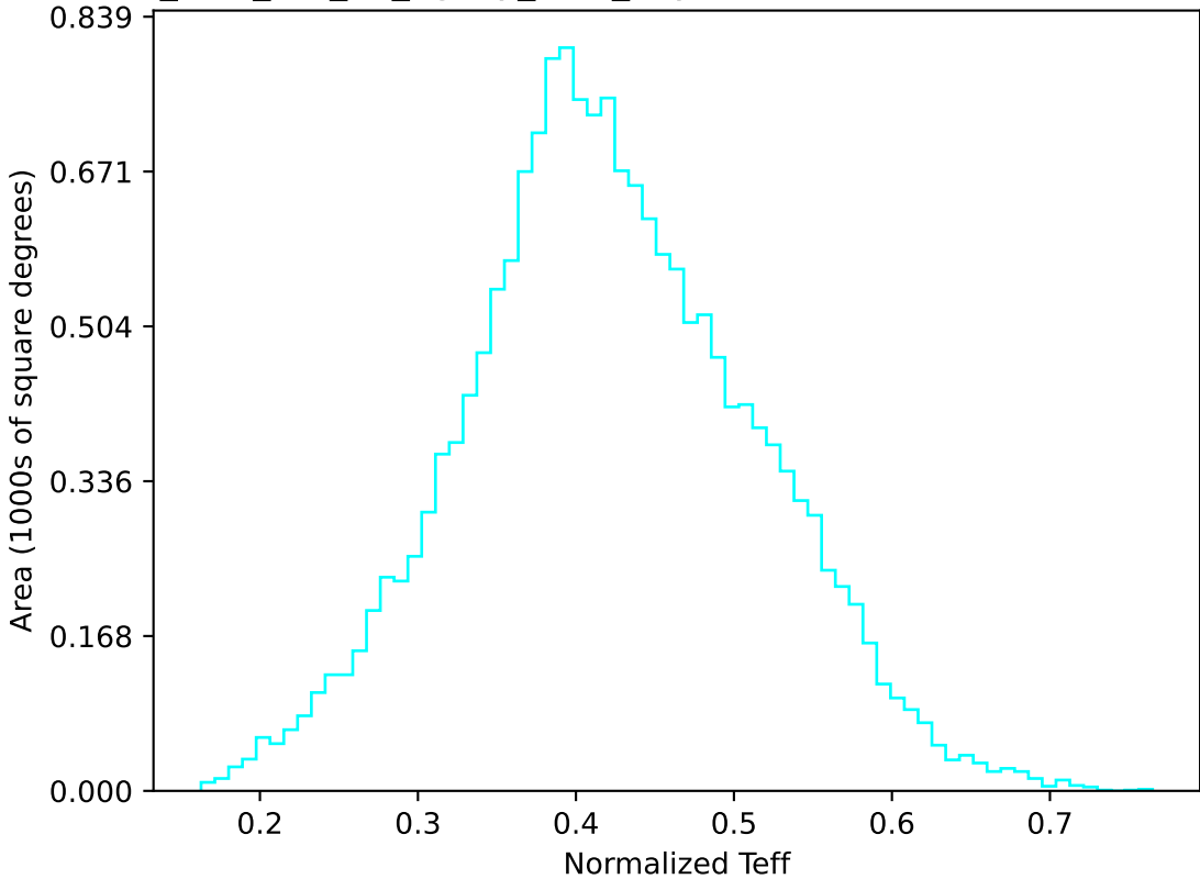
too_elab_r32_d3_ugrizy_v3.4_10yrs WFD u band: Normalized Teff
