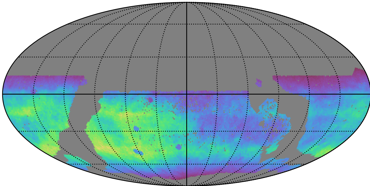
too_elab_r32_d3_ugrizy_v3.4_10yrs WFD r band: Normalized Teff
