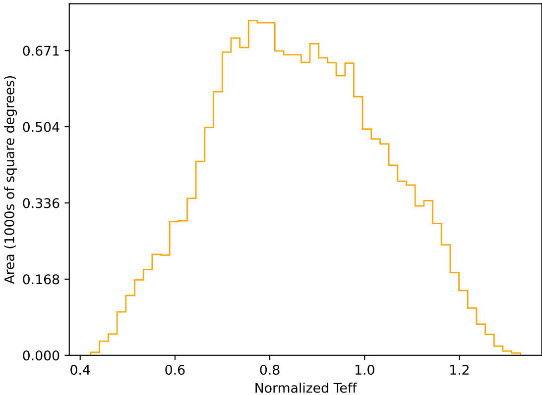
too_elab_r32_d3_ugrizy_v3.4_10yrs WFD r band: Normalized Teff
