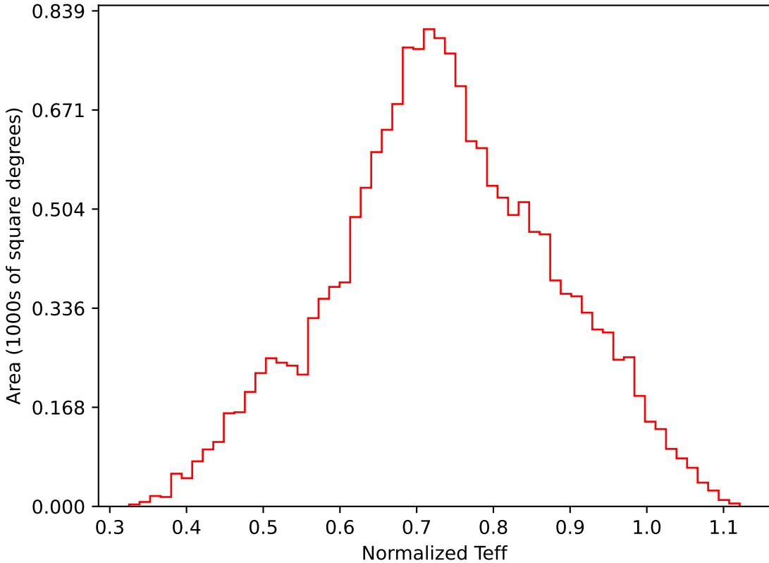
too_elab_r32_d3_ugrizy_v3.4_10yrs WFD i band: Normalized Teff
