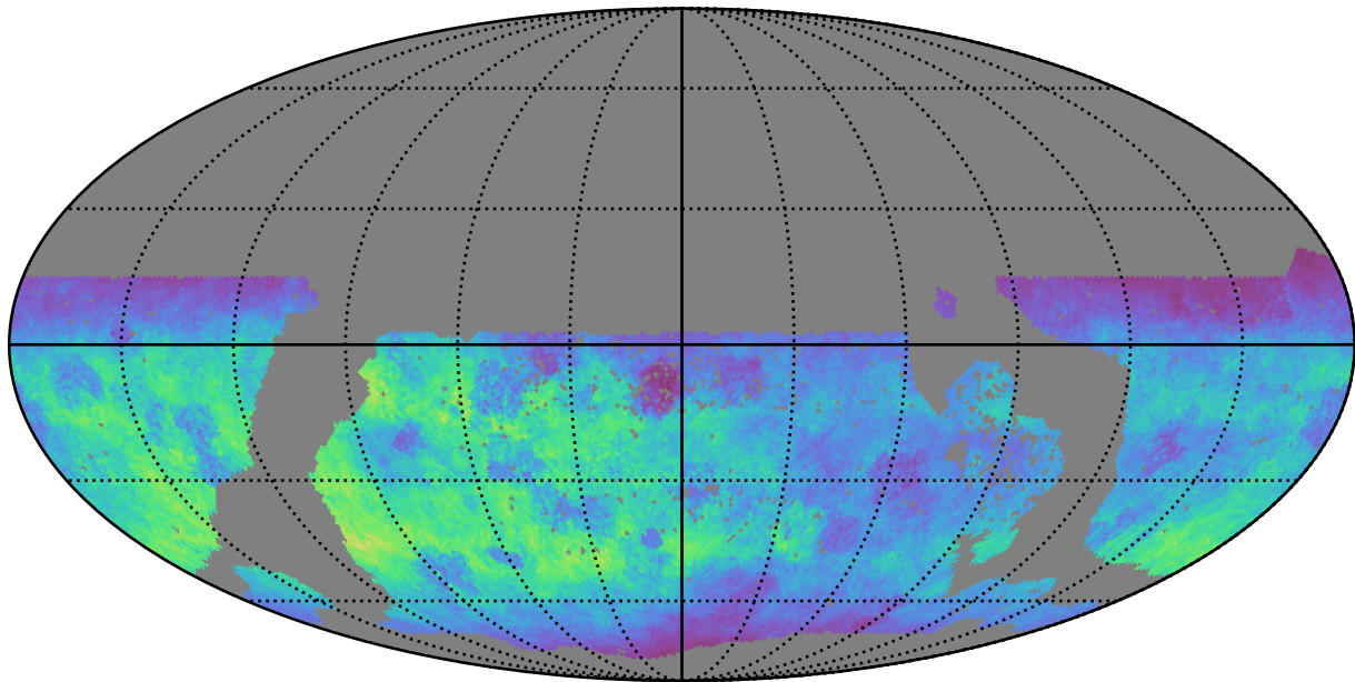
too_elab_r32_d3_ugrizy_v3.4_10yrs WFD g band: Normalized Teff
