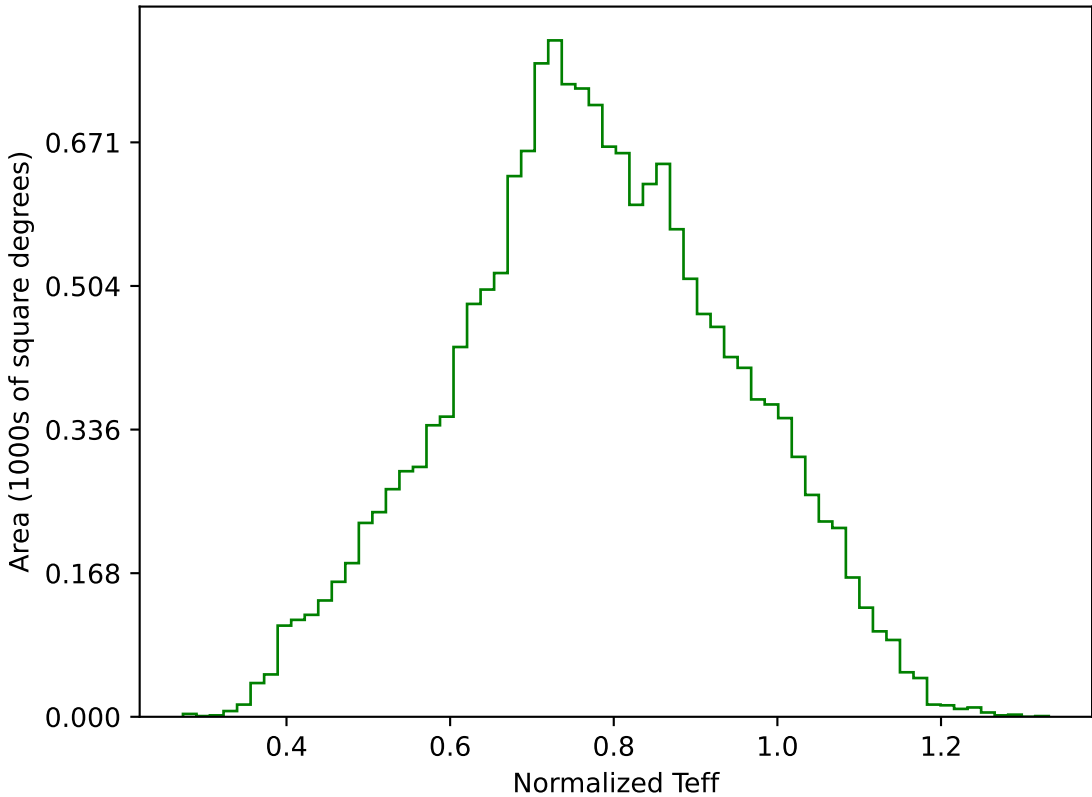
too_elab_r32_d3_ugrizy_v3.4_10yrs WFD g band: Normalized Teff
