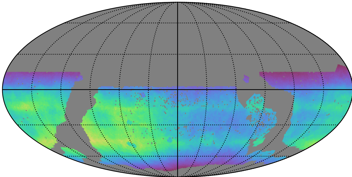
too_elab_r32_d3_ugrizy_v3.4_10yrs WFD all bands: Normalized Teff
