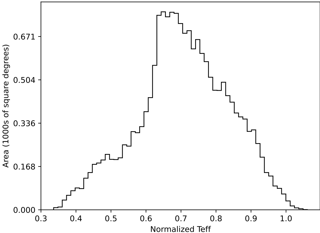
too_elab_r32_d3_ugrizy_v3.4_10yrs WFD all bands: Normalized Teff
