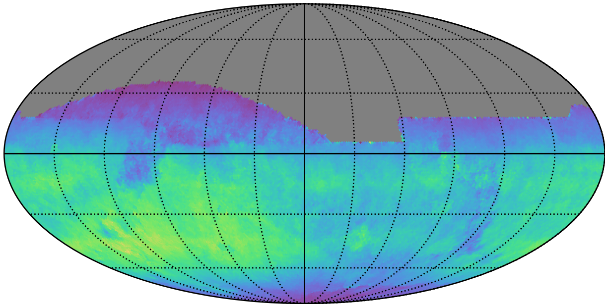
too_elab_r32_d3_ugrizy_v3.4_10yrs All sky z band: Normalized Teff
