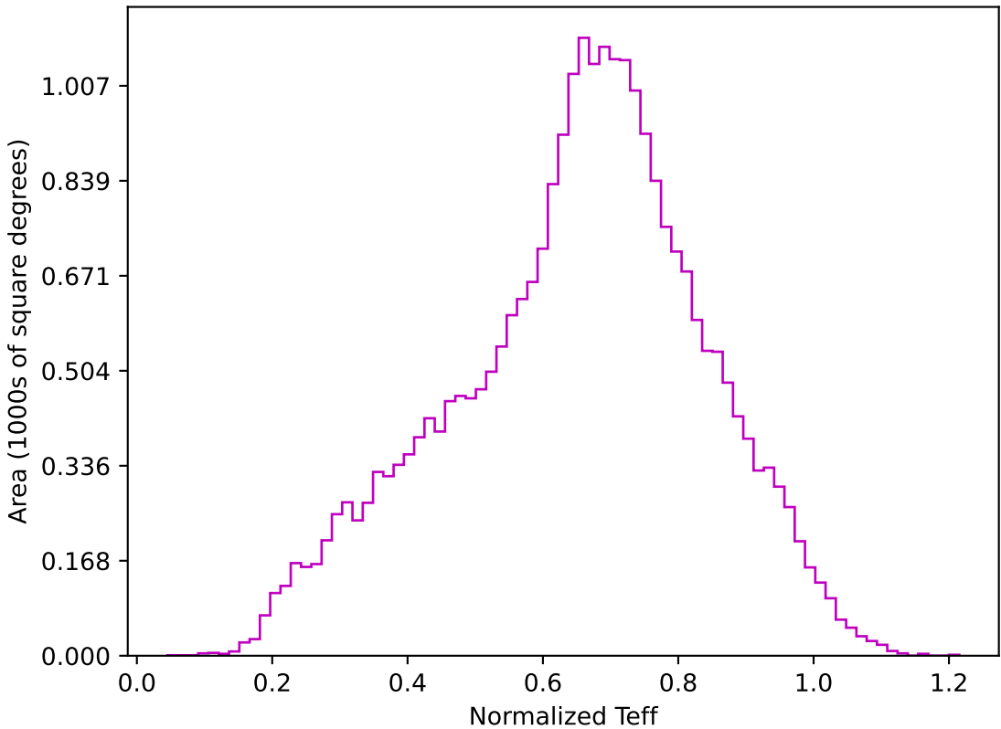
too_elab_r32_d3_ugrizy_v3.4_10yrs All sky z band: Normalized Teff
