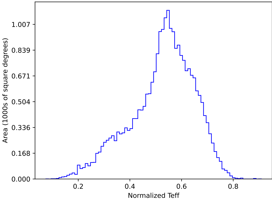
too_elab_r32_d3_ugrizy_v3.4_10yrs All sky y band: Normalized Teff
