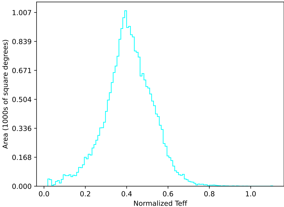
too_elab_r32_d3_ugrizy_v3.4_10yrs All sky u band: Normalized Teff
