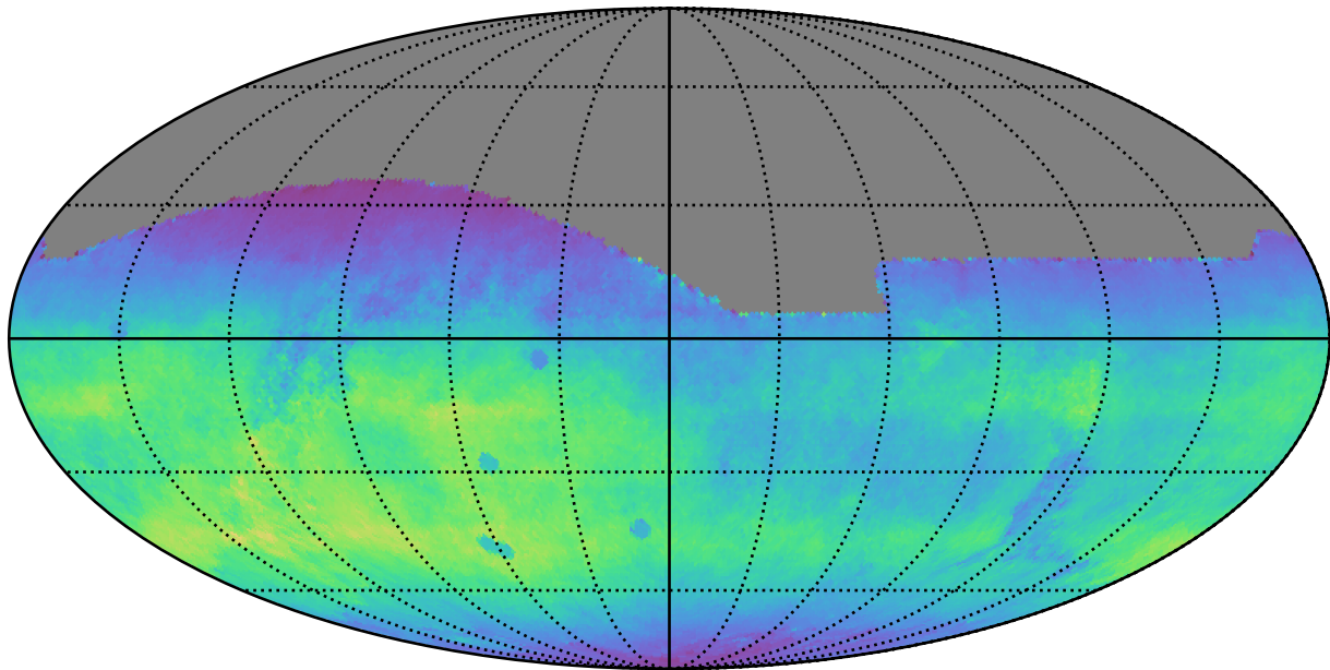
too_elab_r32_d3_ugrizy_v3.4_10yrs All sky r band: Normalized Teff
