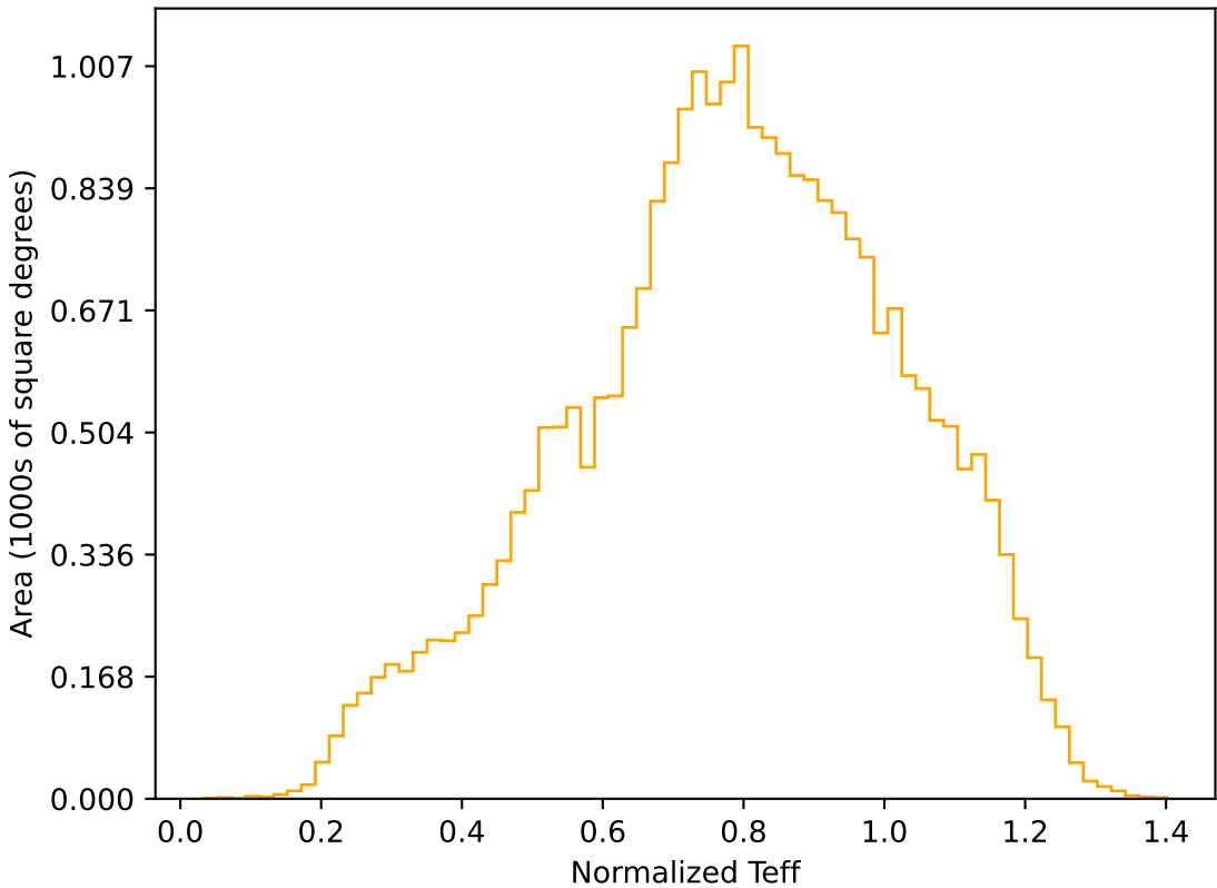
too_elab_r32_d3_ugrizy_v3.4_10yrs All sky r band: Normalized Teff
