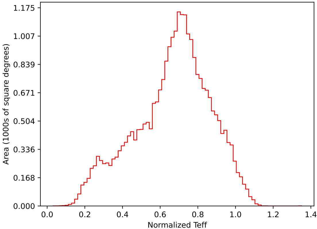
too_elab_r32_d3_ugrizyv3.4_10yrs All sky i band: Normalized Teff
