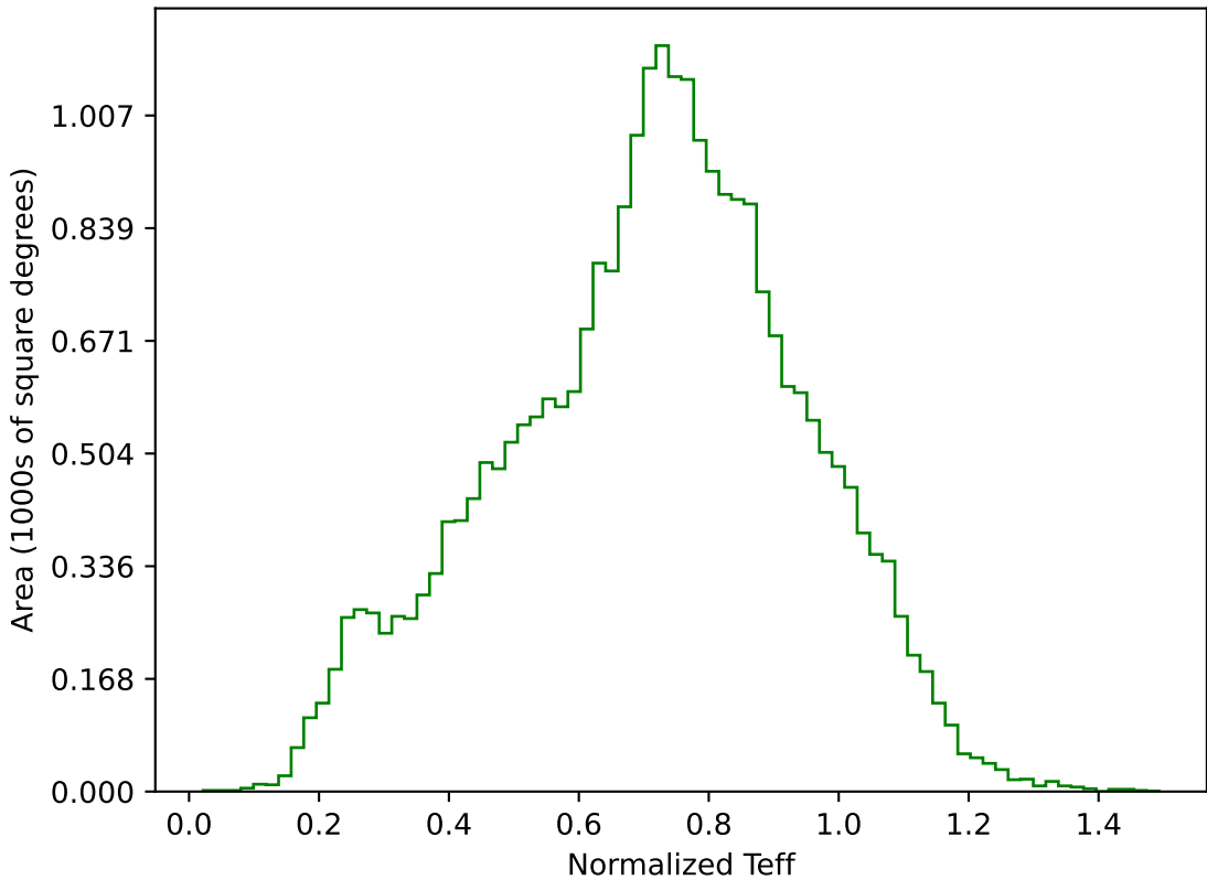
too_elab_r32_d3_ugrizy_v3.4_10yrs All sky g band: Normalized Teff
