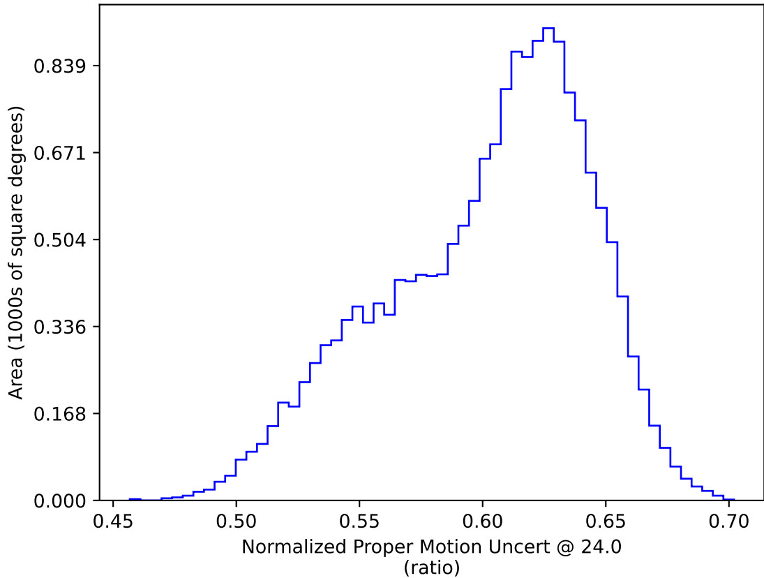
too_elab_r32_d3_ugrizy_v3.4_10yrs WFD: Normalized Proper Motion Uncert @ 24.0
