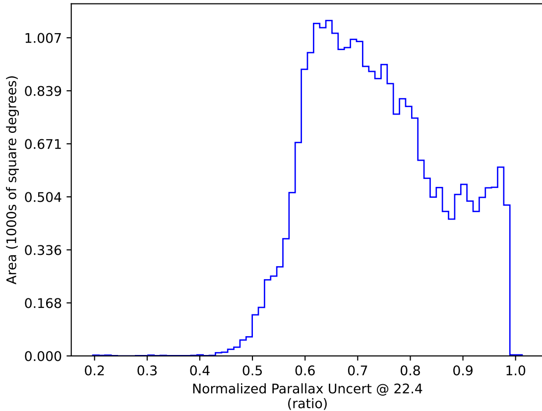
too_elab_r32_d3_ugrizy_v3.4_10yrs All sky: Normalized Parallax Uncert @ 22.4
