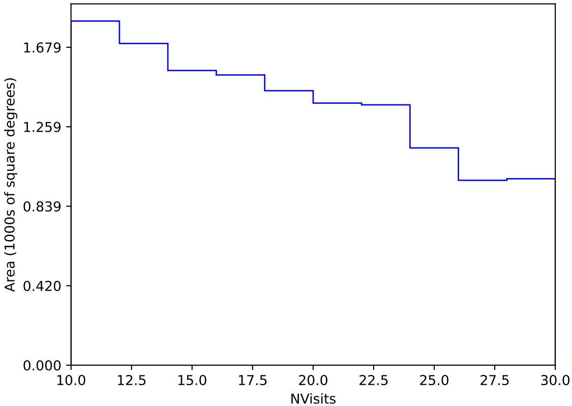
too_elab_r32_d3_ugrizy_v3.4_10yrs Yr 3-4 y band: NVisits
