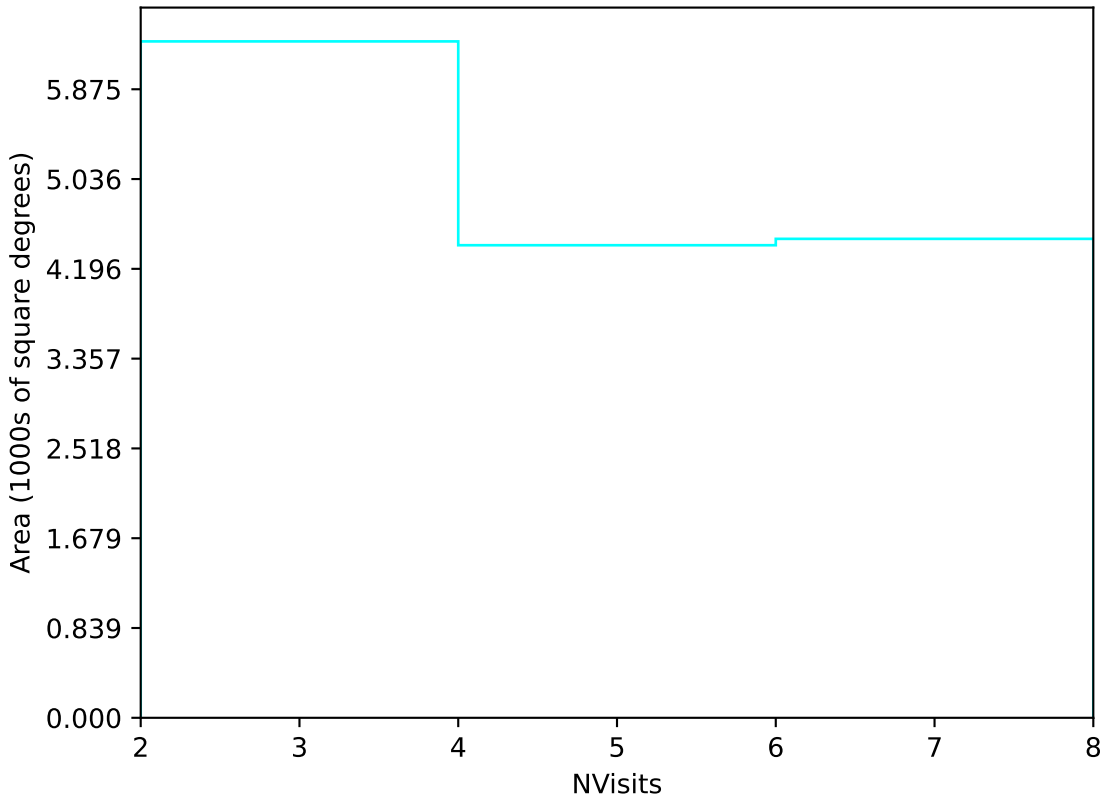
too_elab_r32_d3_ugrizy_v3.4_10yrs Yr 3-4 u band: NVisits
