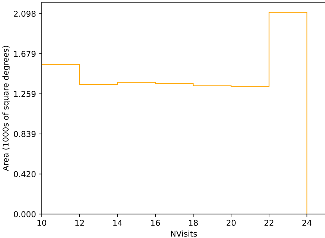
too_elab_r32_d3_ugrizy_v3.4_10yrs Yr 3-4 r band: NVisits
