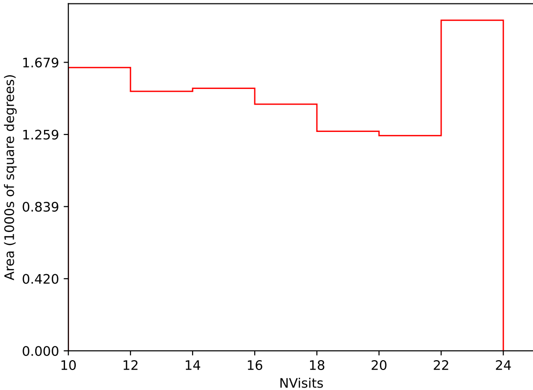
too_elab_r32_d3_ugrizy_v3.4_10yrs Yr 3-4 i band: NVisits
