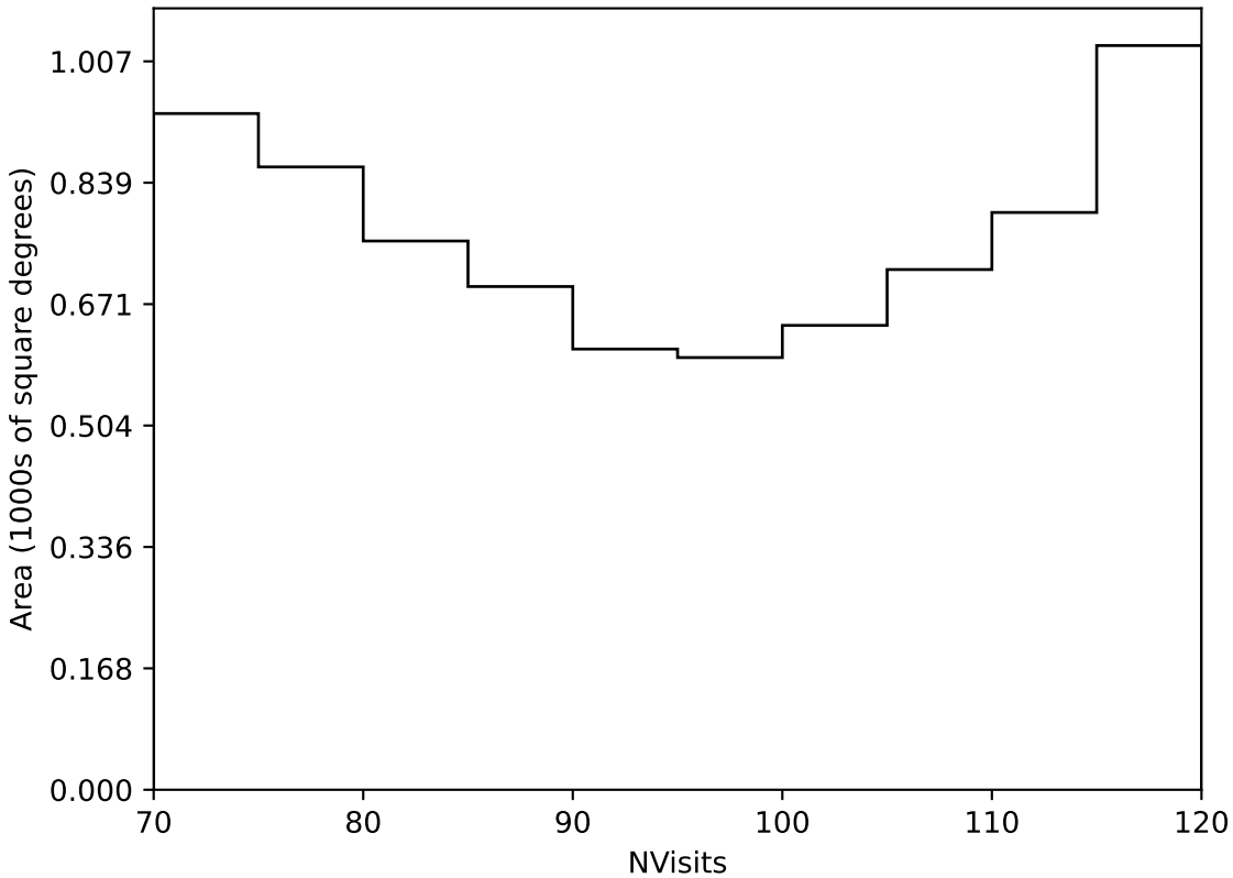
too_elab_r32_d3_ugrizy_v3.4_10yrs Yr 3-4 all bands: NVisits
