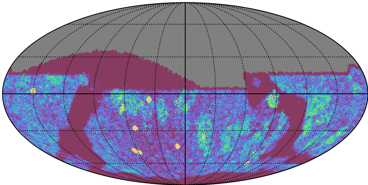
too_elab_r32_d3_ugrizy_v3.4_10yrs Yr 1 z band: NVisits
