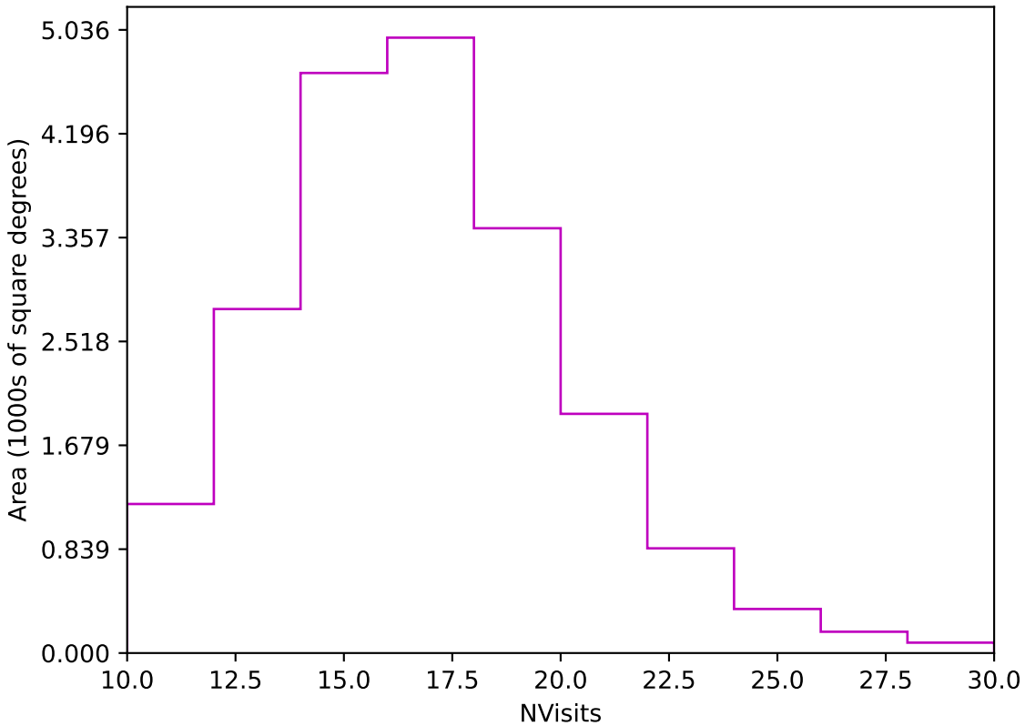
too_elab_r32_d3_ugrizy_v3.4_10yrs Yr 1 z band: NVisits
