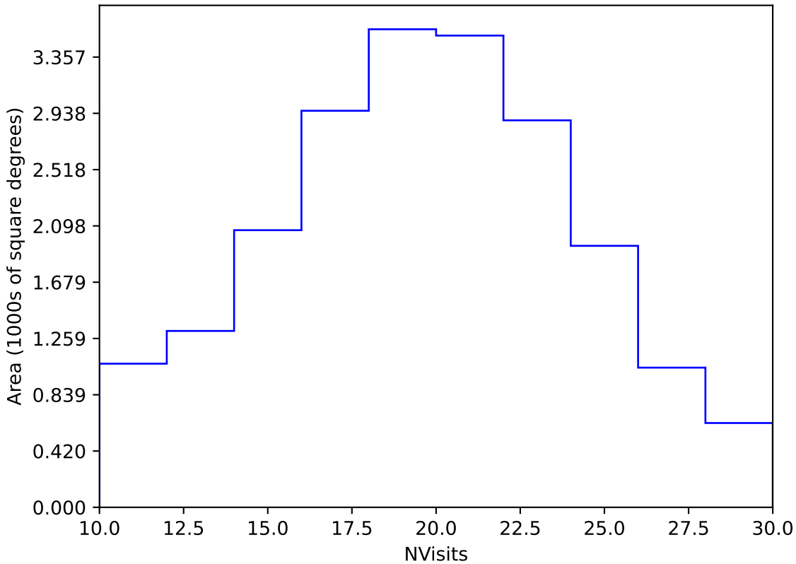
too_elab_r32_d3_ugrizy_v3.4_10yrs Yr 1 y band: NVisits
