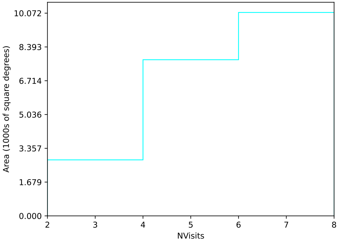
too_elab_r32_d3_ugrizy_v3.4_10yrs Yr 1 u band: NVisits
