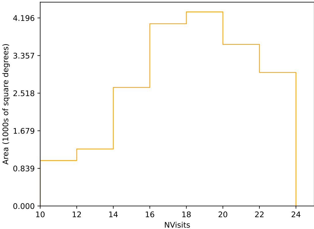
too_elab_r32_d3_ugrizy_v3.4_10yrs Yr 1 r band: NVisits
