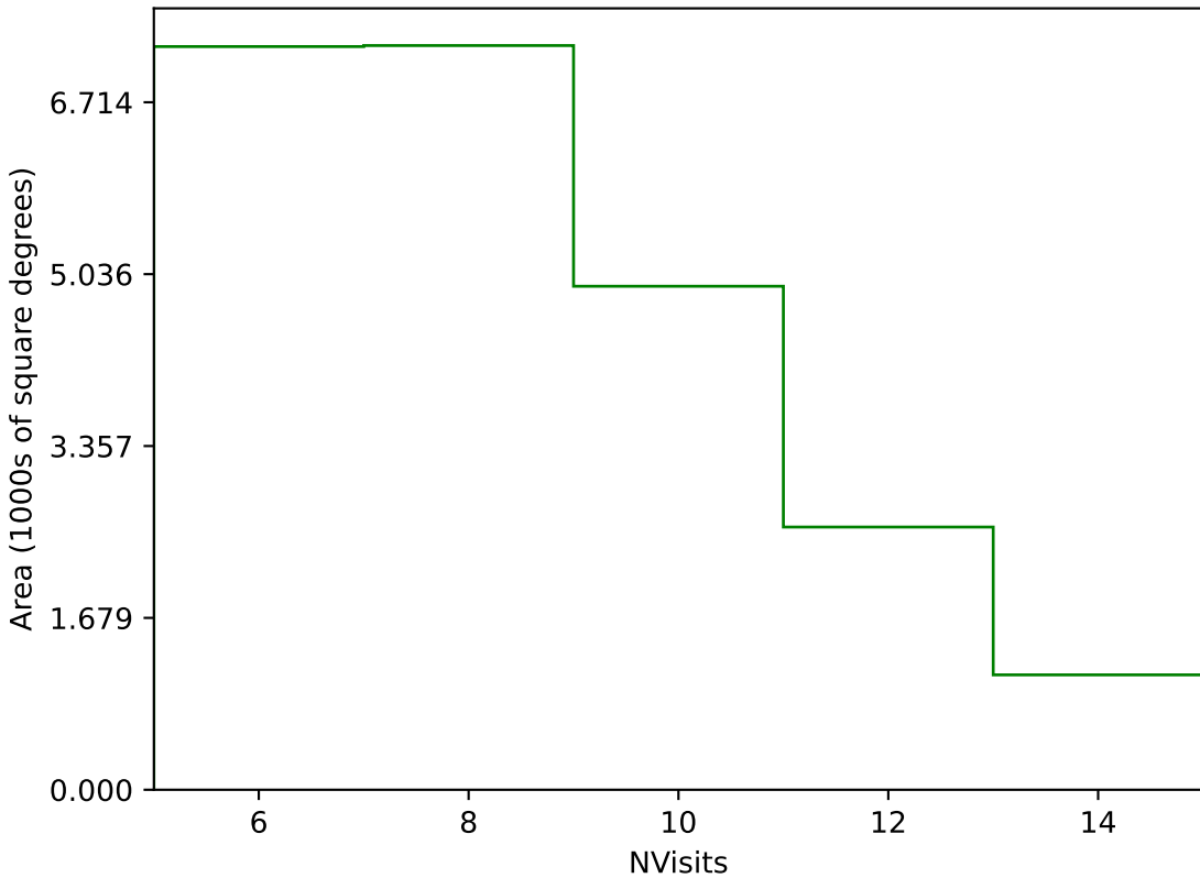
too_elab_r32_d3_ugrizy_v3.4_10yrs Yr 1 g band: NVisits
