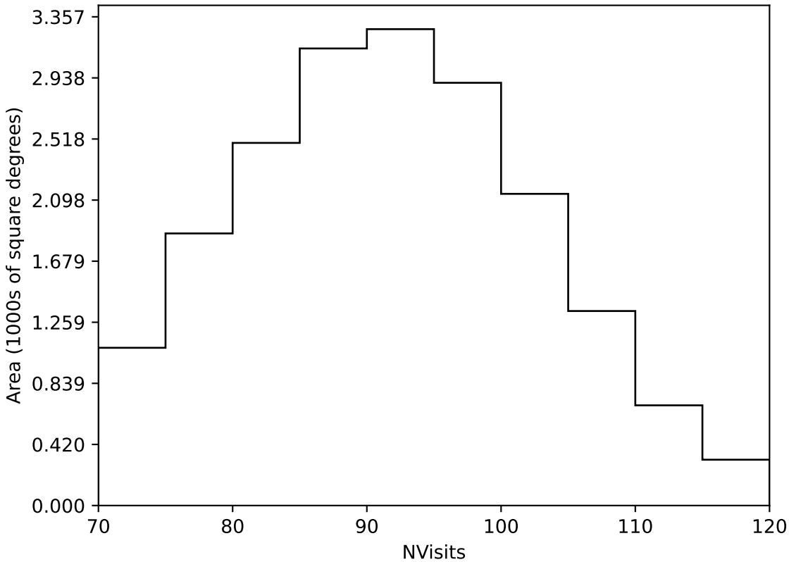
too_elab_r32_d3_ugrizy_v3.4_10yrs Yr 1 all bands: NVisits
