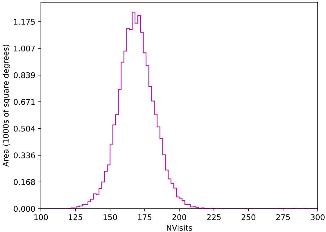
too_elab_r32_d3_ugrizy_v3.4_10yrs WFD z band: NVisits
