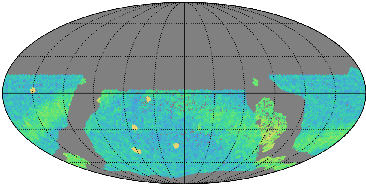
too_elab_r32_d3_ugrizy_v3.4_10yrs WFD r band: NVisits
