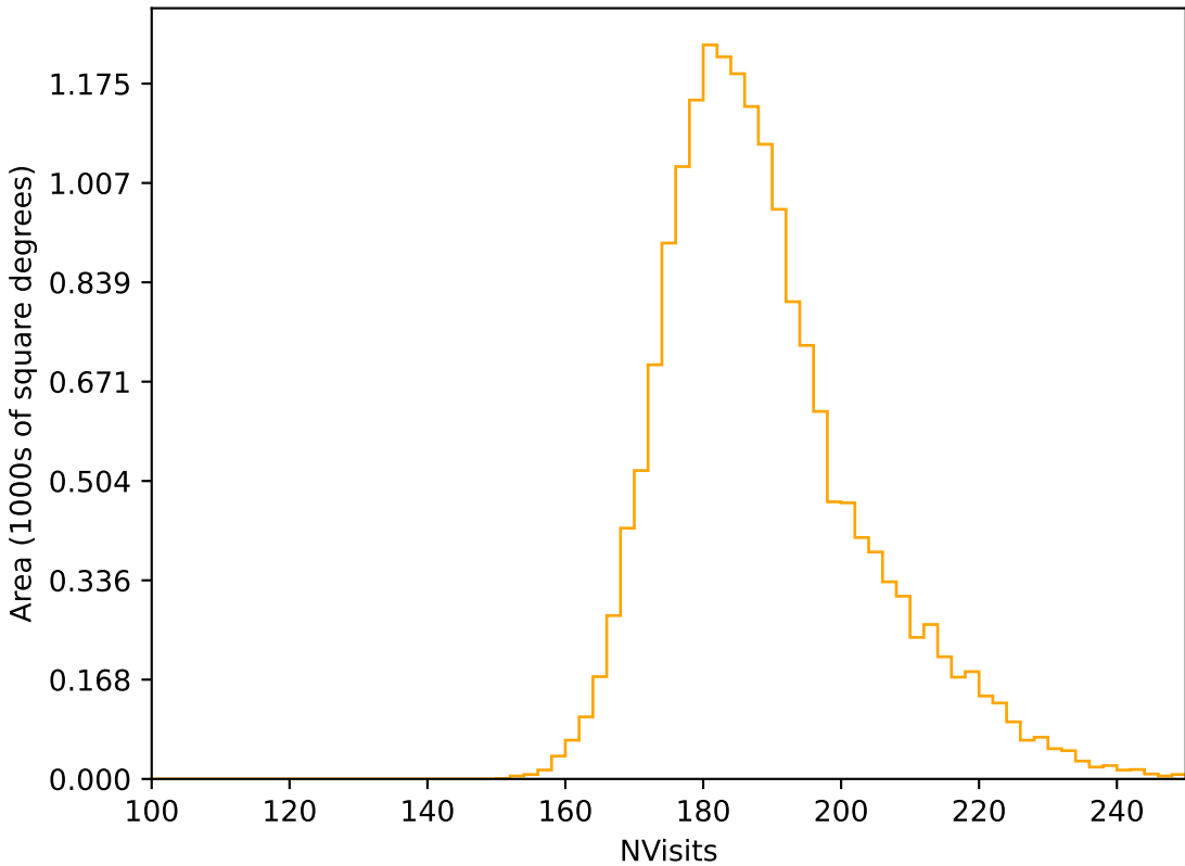
too_elab_r32_d3_ugrizy_v3.4_10yrs WFD r band: NVisits
