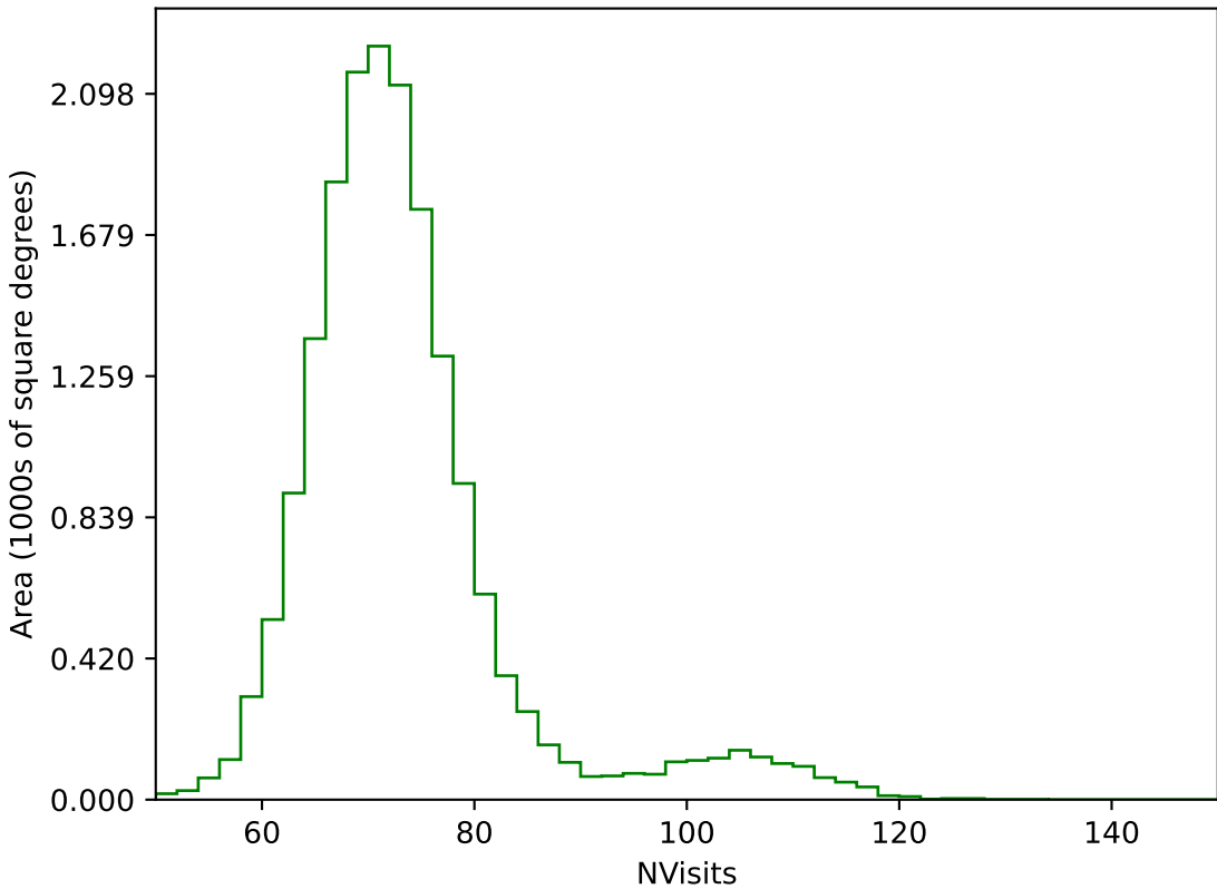
too_elab_r32_d3_ugrizy_v3.4_10yrs WFD g band: NVisits
