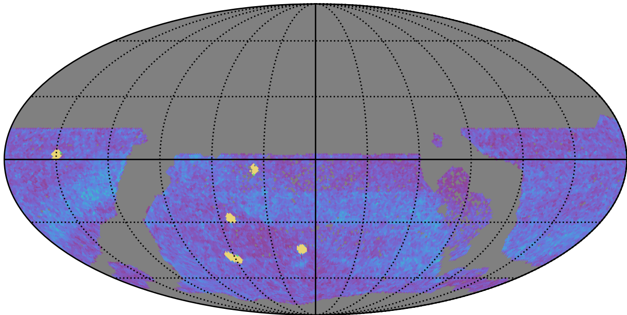
too_elab_r32_d3_ugrizy_v3.4_10yrs WFD all bands: NVisits
