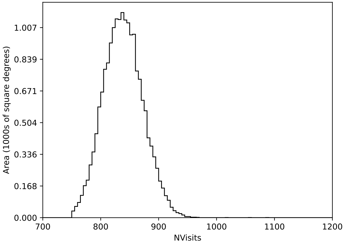
too_elab_r32_d3_ugrizy_v3.4_10yrs WFD all bands: NVisits
