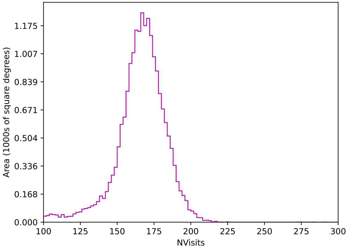
too_elab_r32_d3_ugrizy_v3.4_10yrs All sky z band: NVisits
