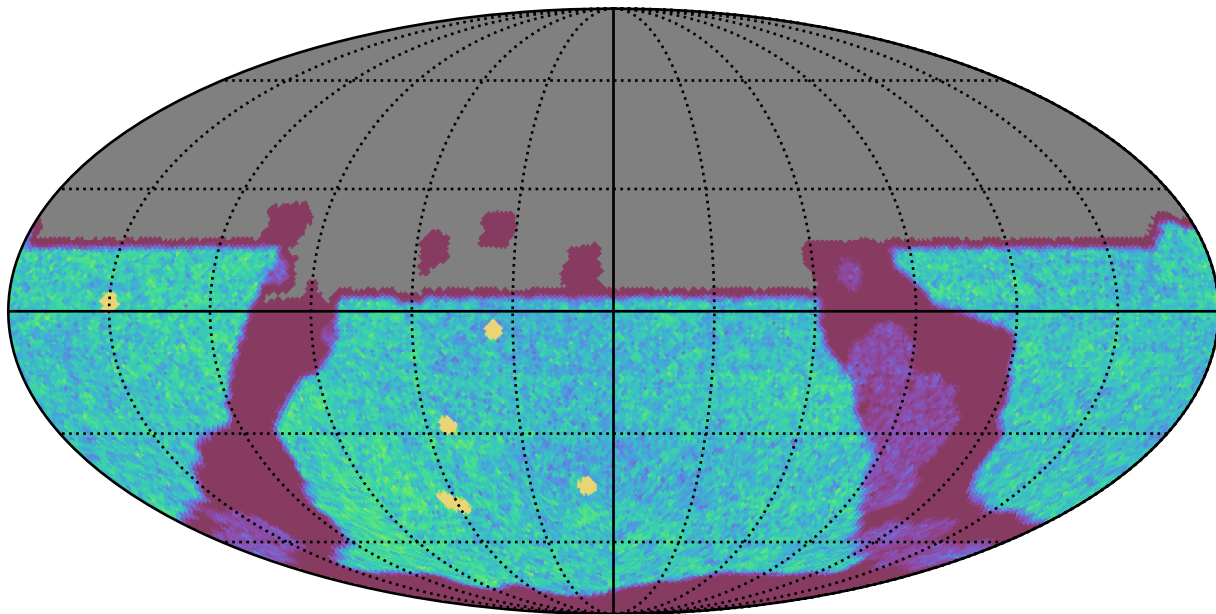
too_elab_r32_d3_ugrizy_v3.4_10yrs All sky u band: NVisits
