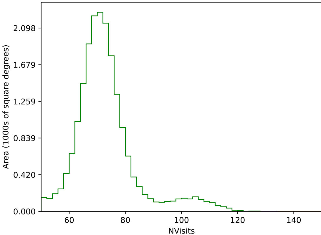
too_elab_r32_d3_ugrizy_v3.4_10yrs All sky g band: NVisits
