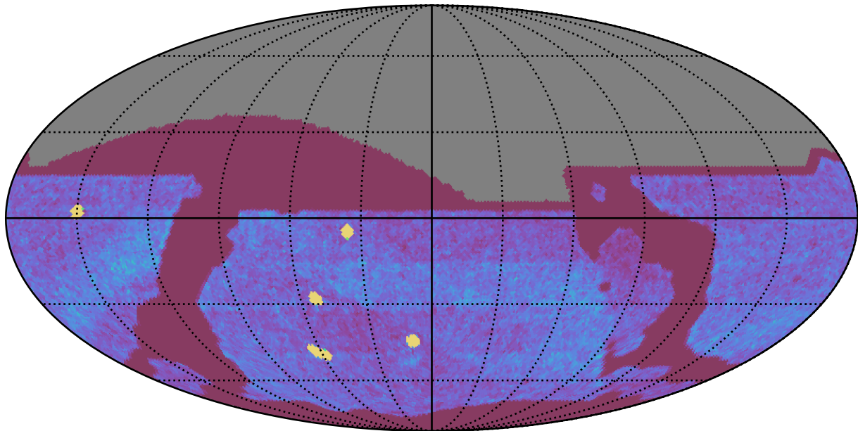
too_elab_r32_d3_ugrizy_v3.4_10yrs All sky all bands: NVisits
