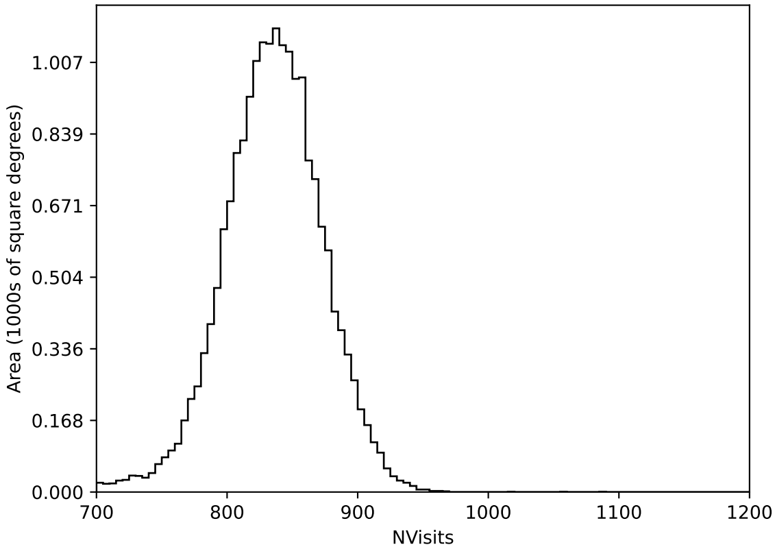
too_elab_r32_d3_ugrizy_v3.4_10yrs All sky all bands: NVisits
