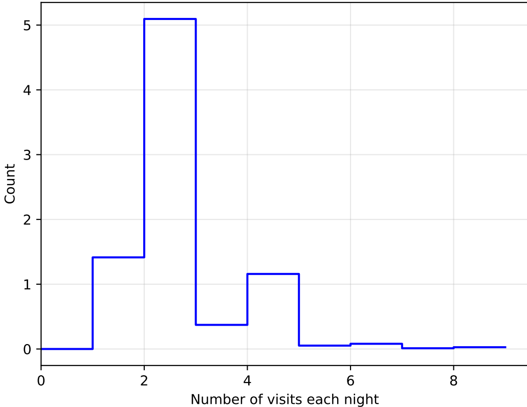
too_elab_r32_d3_ugrizy_v3.4_10yrs WFD: NVisitsPerNight 1e6
