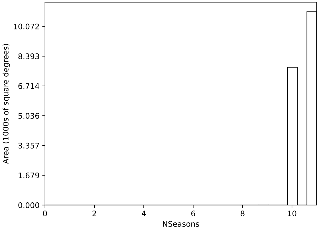
too_elab_r32_d3_ugrizy_v3.4_10yrs WFD all bands: NSeasons
