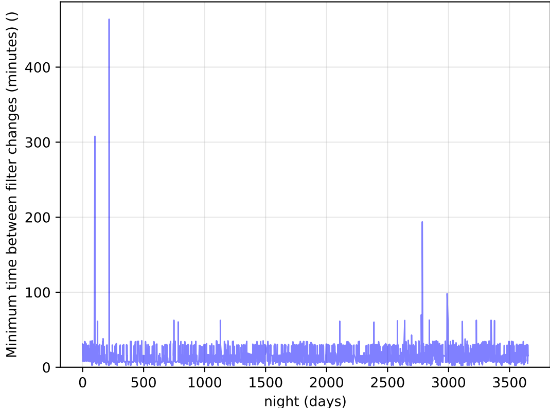
too_elab_r32_d3_ugrizy_v3.4_10yrs Per Night: Minimum time between filter changes (minutes)
