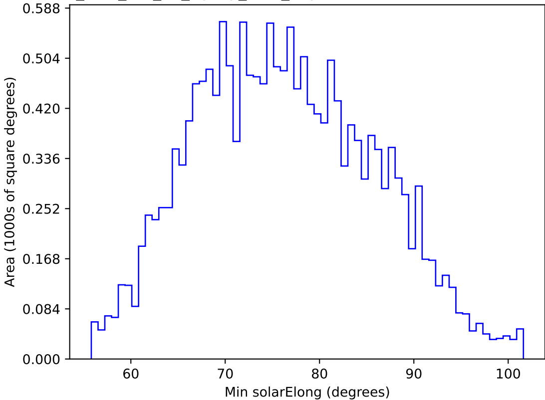
too_elab_r32_d3_ugrizy_v3.4_10yrs WFD u band: Min solarElong
