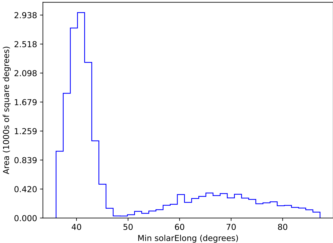
too_elab_r32_d3_ugrizy_v3.4_10yrs WFD i band: Min solarElong
