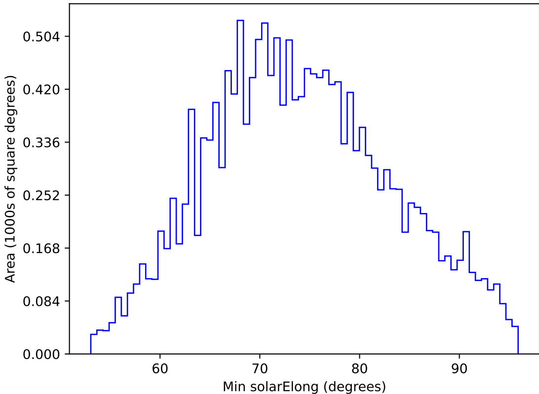
too_elab_r32_d3_ugrizy_v3.4_10yrs WFD g band: Min solarElong
