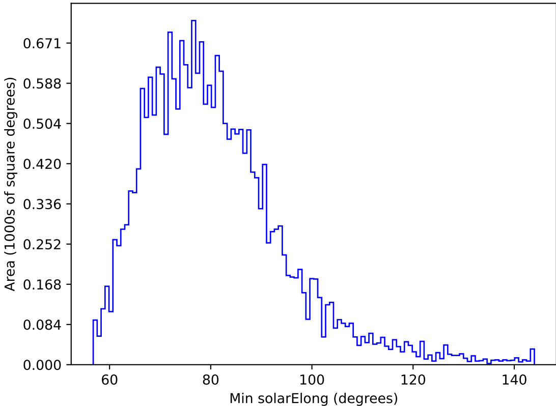
too_elab_r32_d3_ugrizy_v3.4_10yrs All sky u band: Min solarElong
