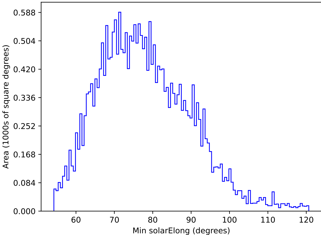
too_elab_r32_d3_ugrizy_v3.4_10yrs All sky g band: Min solarElong
